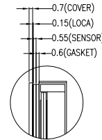
DETAIL B SCALE 2:1
